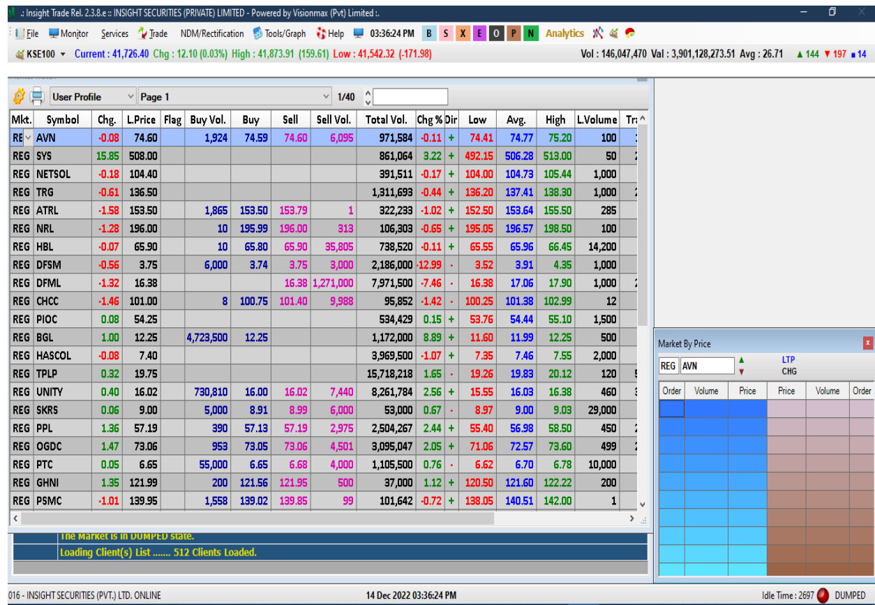
Fig 3 - Main Window
